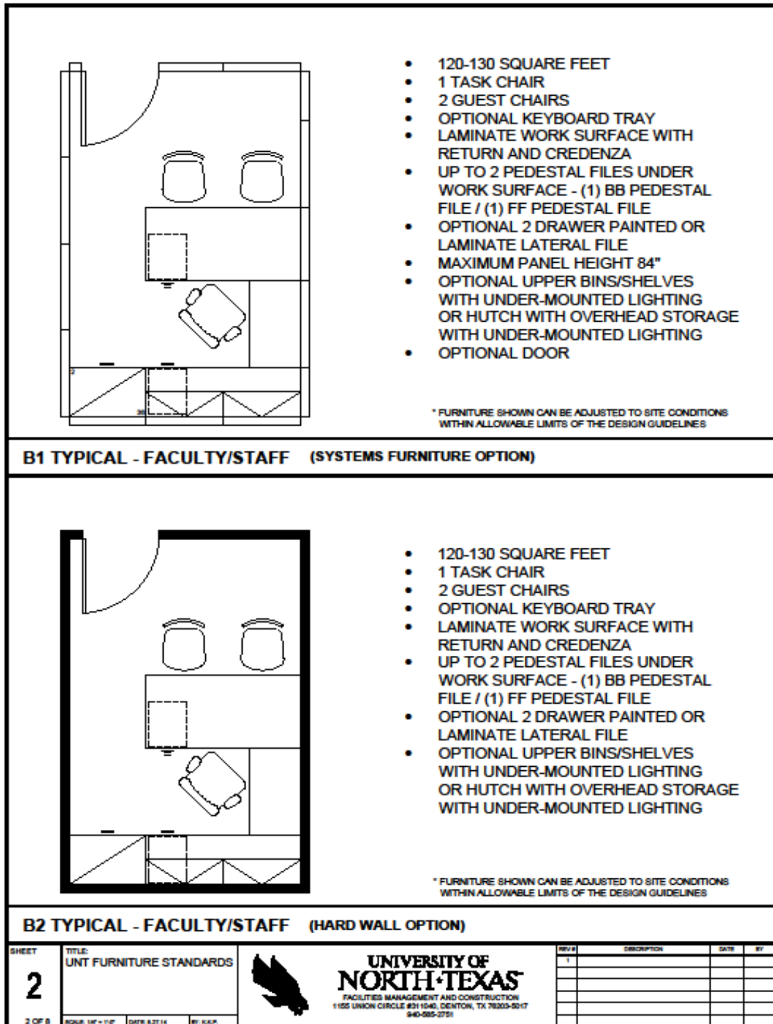
Figure 26 Office Standards: Typical B
