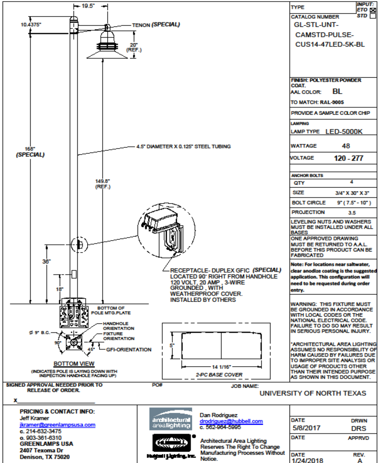
Figure 38 Standard Light Pole Specification
