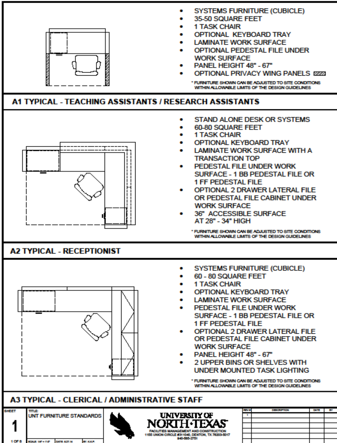
Figure 25 Office Standards: Typical A
