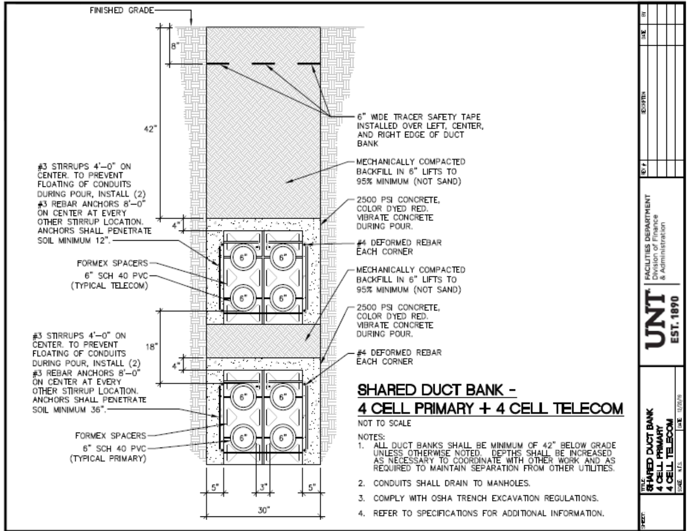
Figure 46 Shared Duct bank 4 Cell Primary & 4 Cell Telecom
