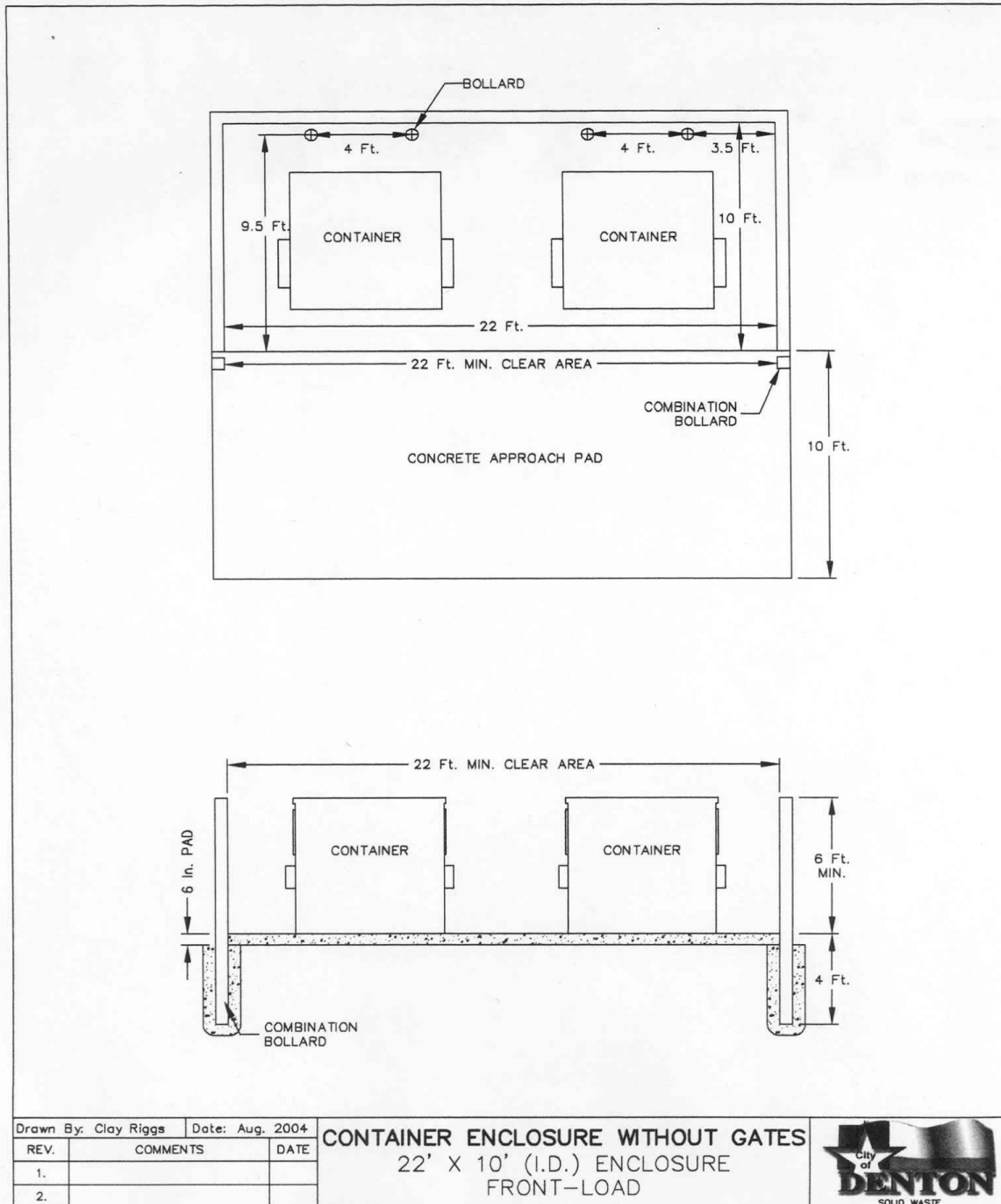
Figure 10 Outdoor Solid Waste Container Enclosure Without Gates Detail
