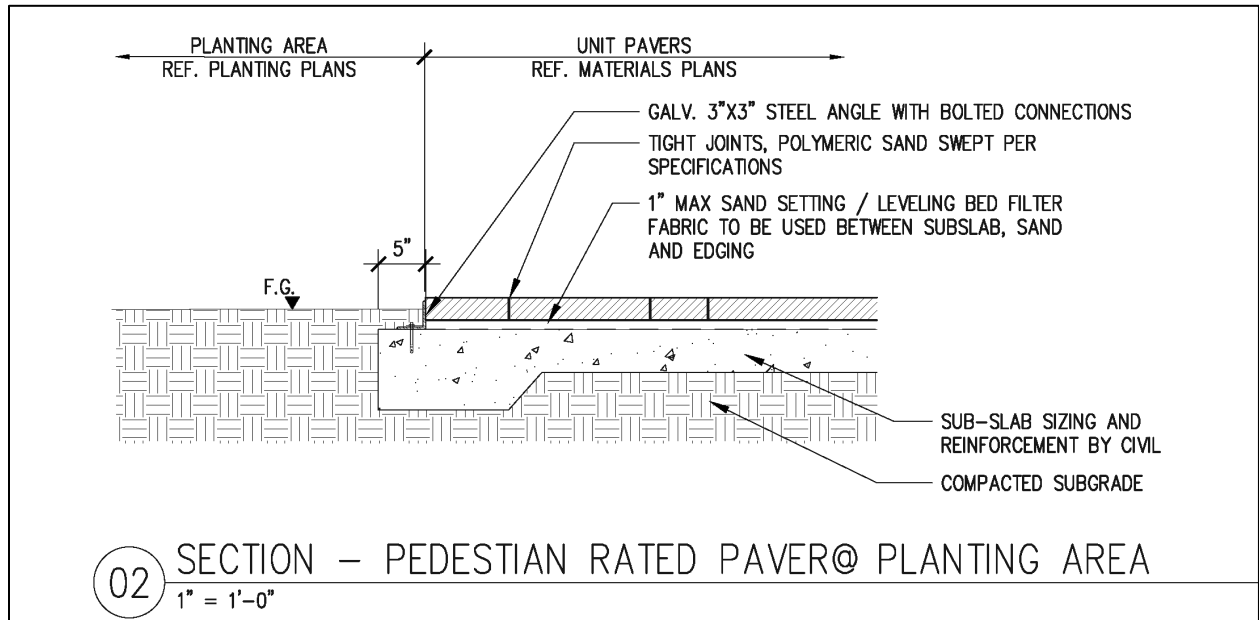
Figure 52 Paver Design
