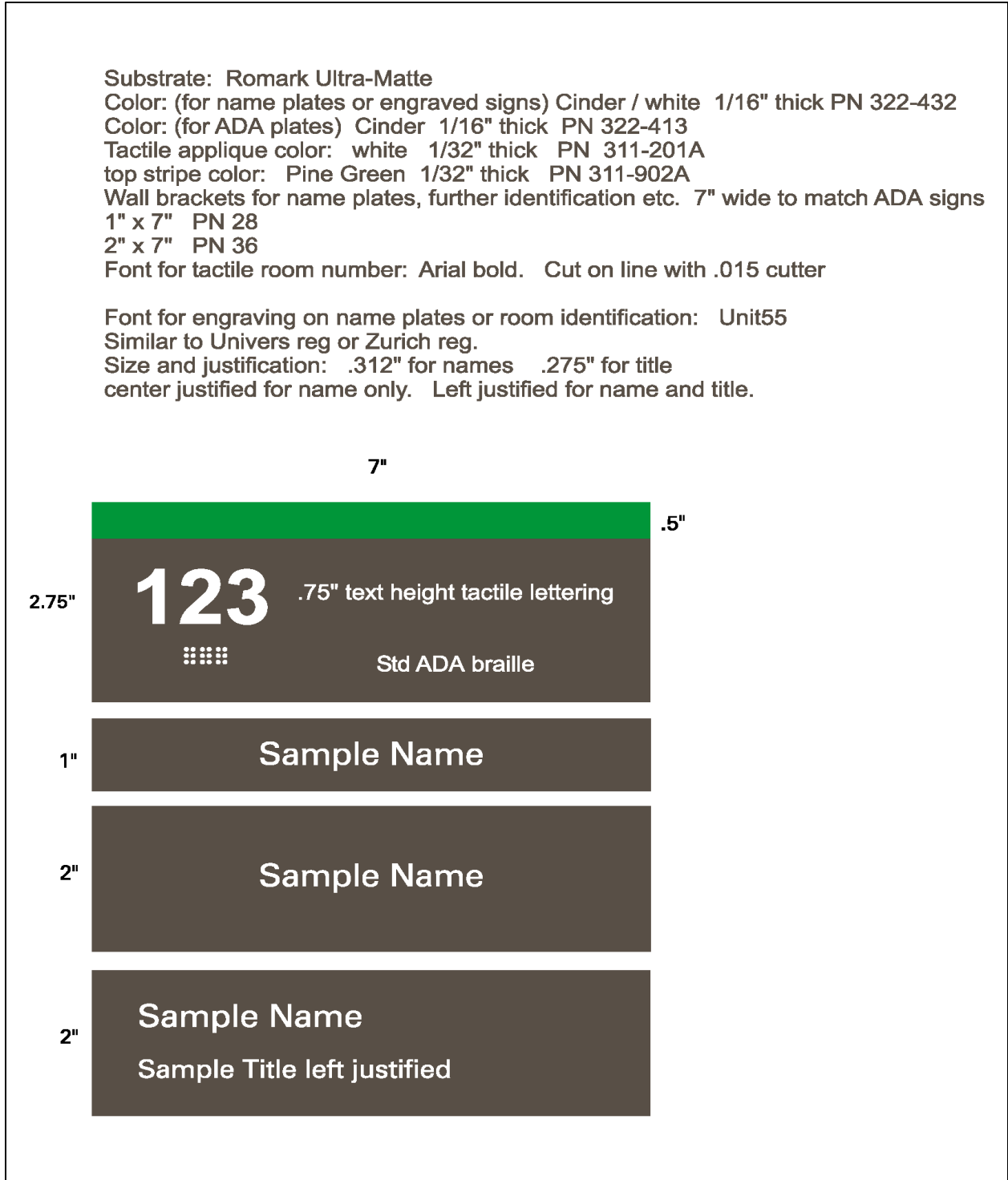
Figure 17 Interior Signage Plate Details Option 1 Renovation to match adjacent
