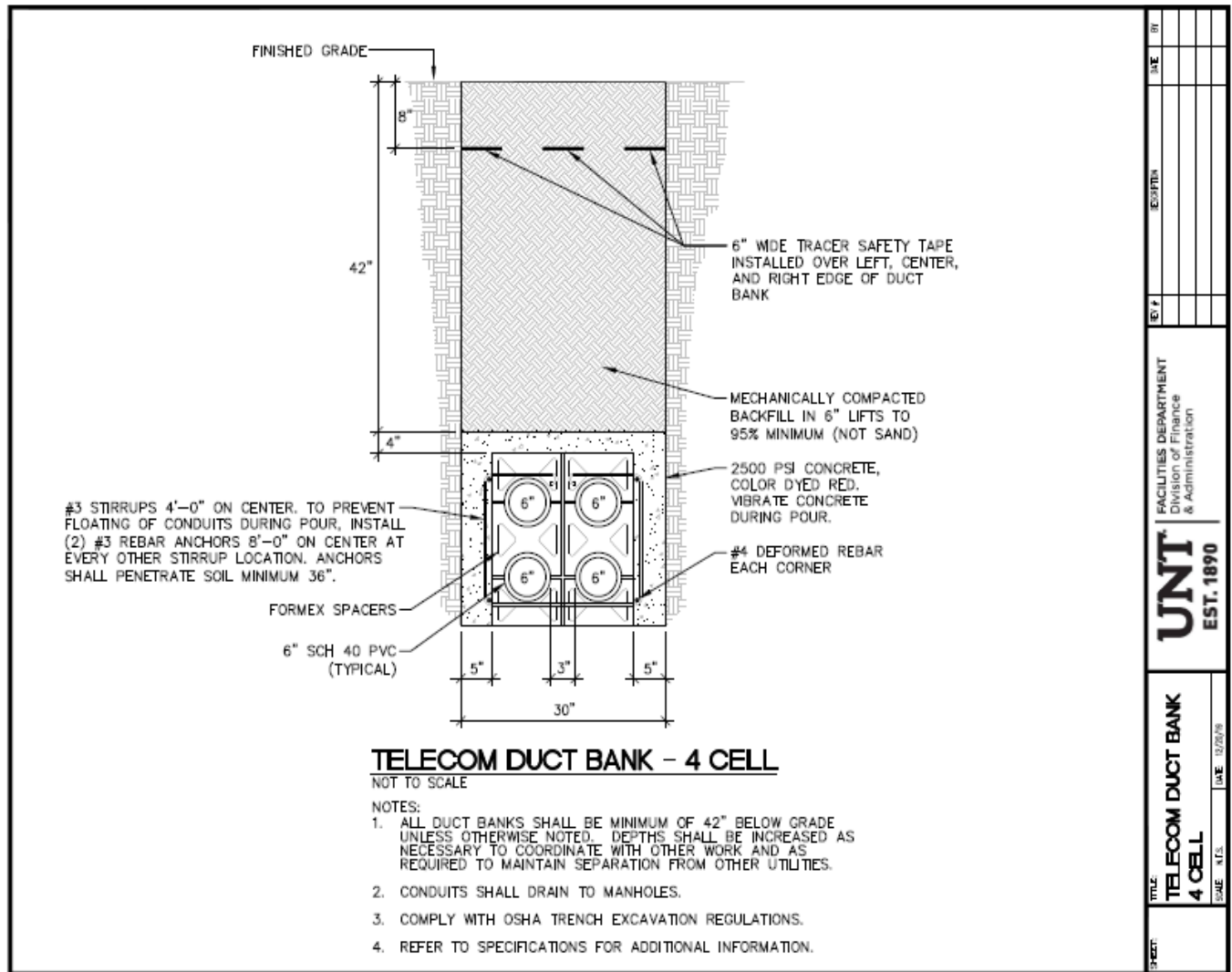
Figure 45 Telecommunications Duct Bank 4 Cell
