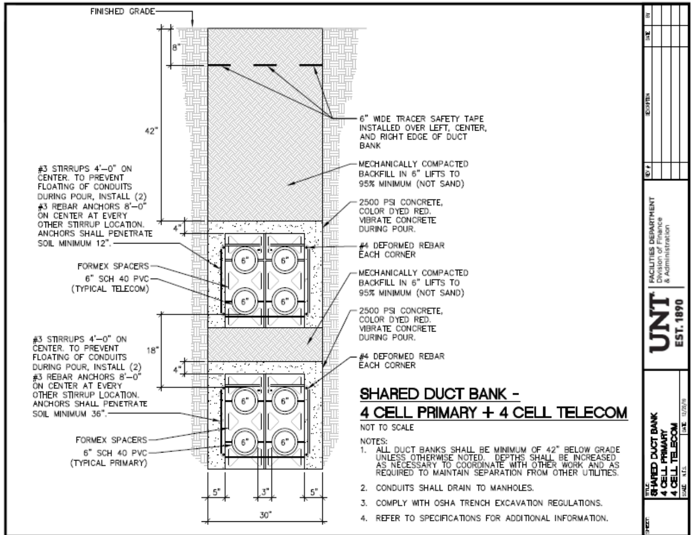
Figure 46 Shared Duct bank 4 Cell Primary &amp; 4 Cell Telecom
