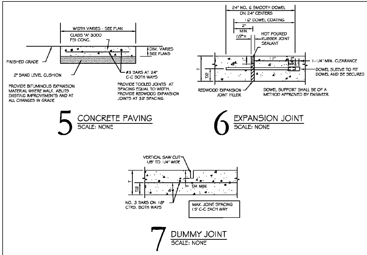
Figure 51 Control and Expansion Joints
