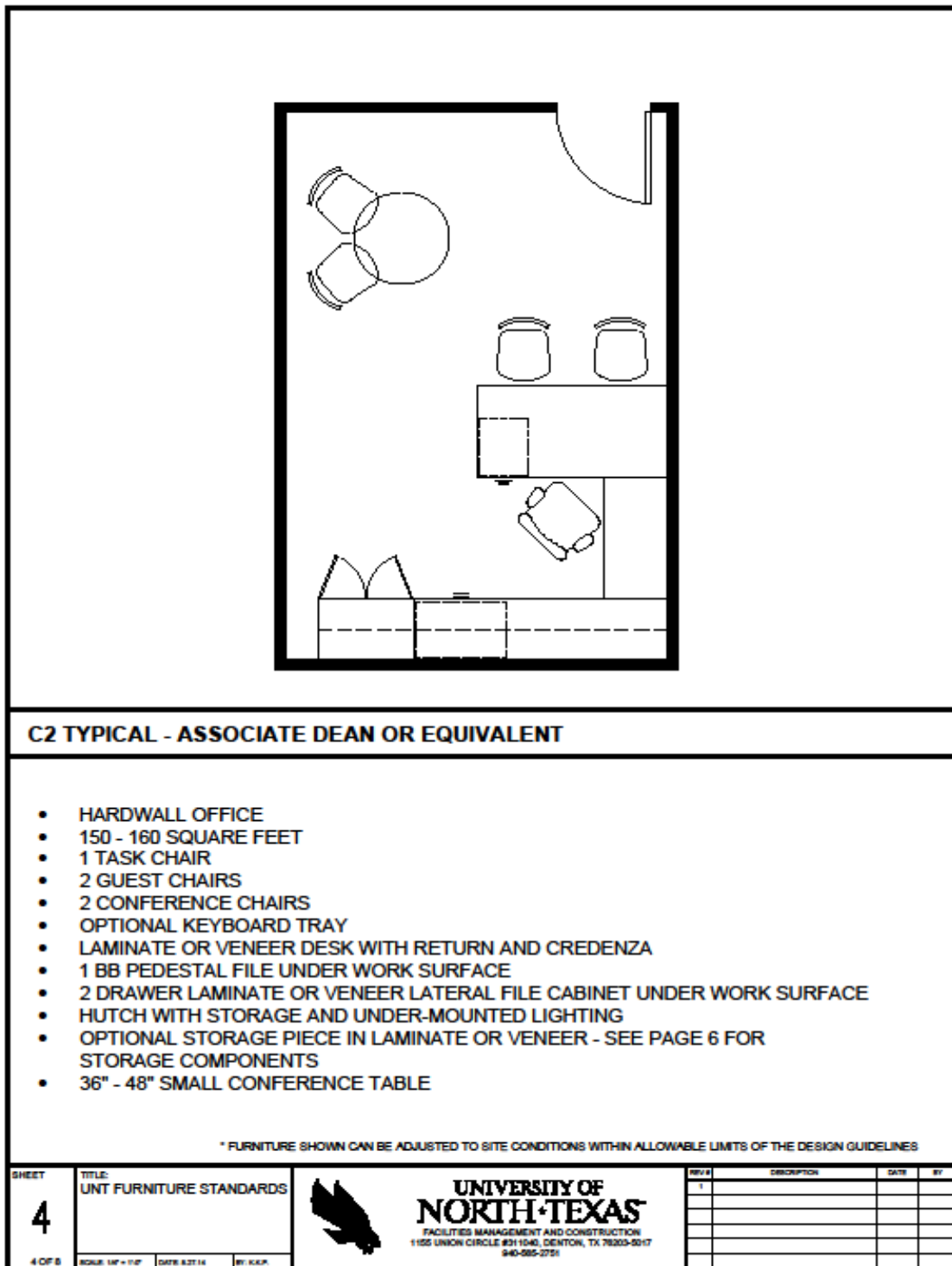
Figure 28 Office Standards: Typical C2
