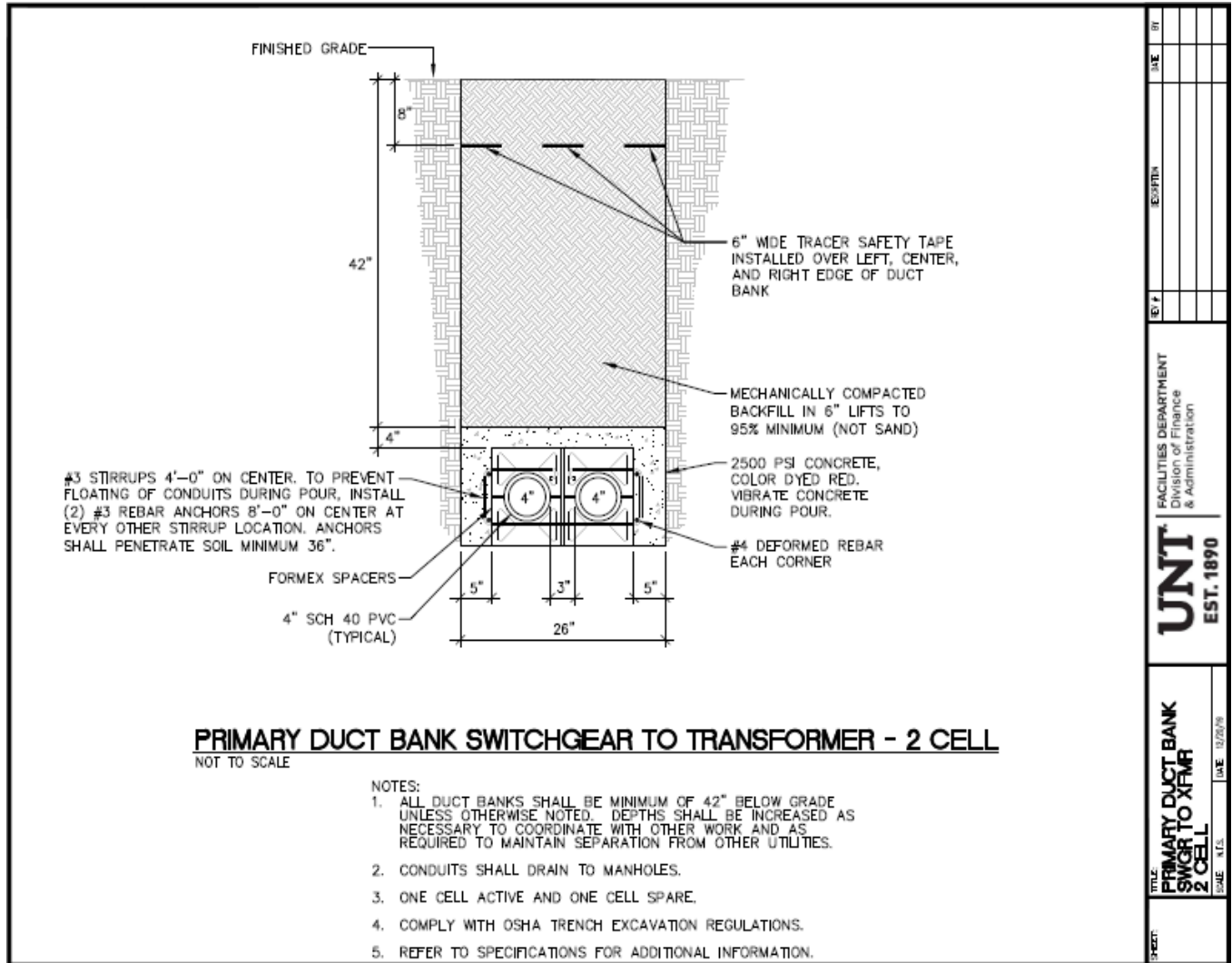
Figure 42 Primary Power Duct bank 2-Cell to Transformer
