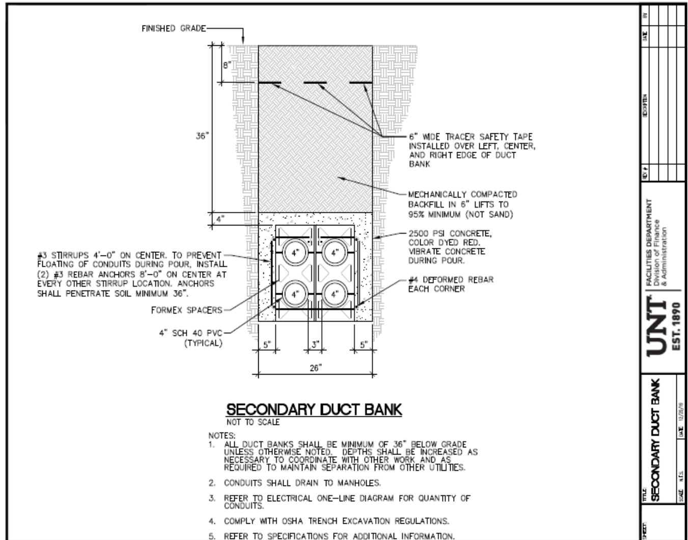
Figure 43 Secondary Power Duct Bank
