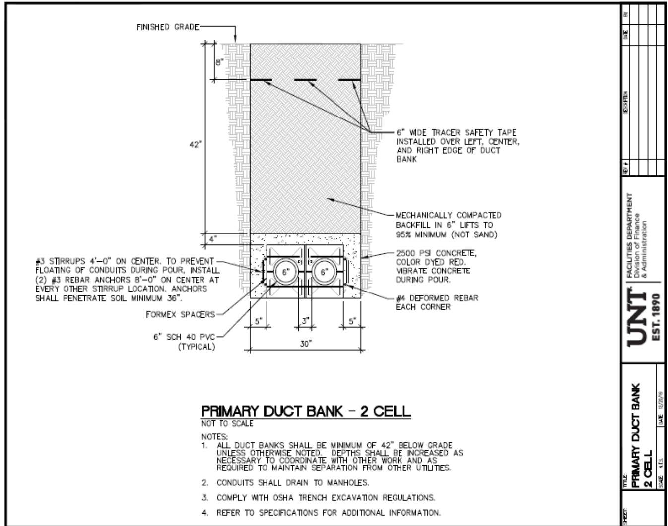
Figure 41 Primary Power Duct Bank 2-Cell
