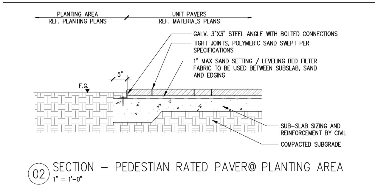
Figure 50 Paver Design
