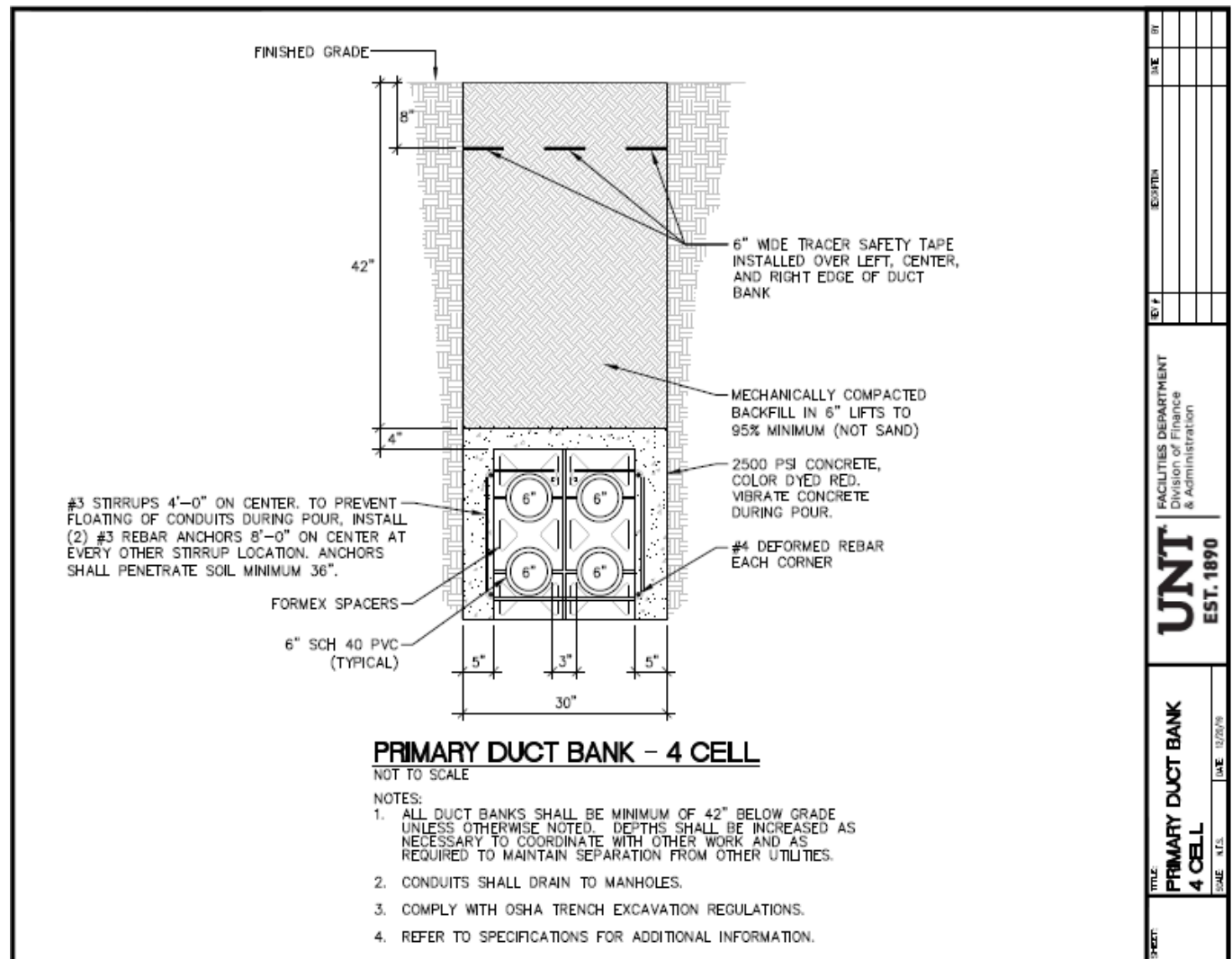
Figure 40 Primary Power Duct bank 4-Cell
