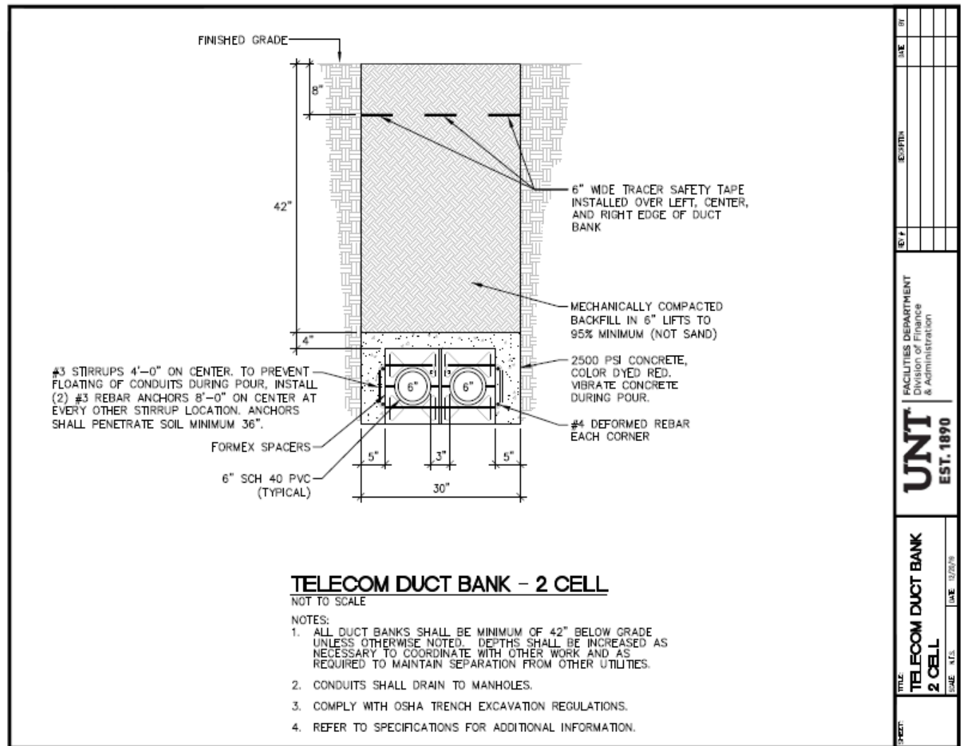
Figure 44 Telecommunications Duct bank
