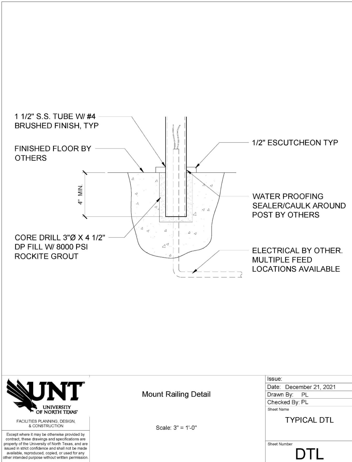
Figure 34 Handrail Detail
