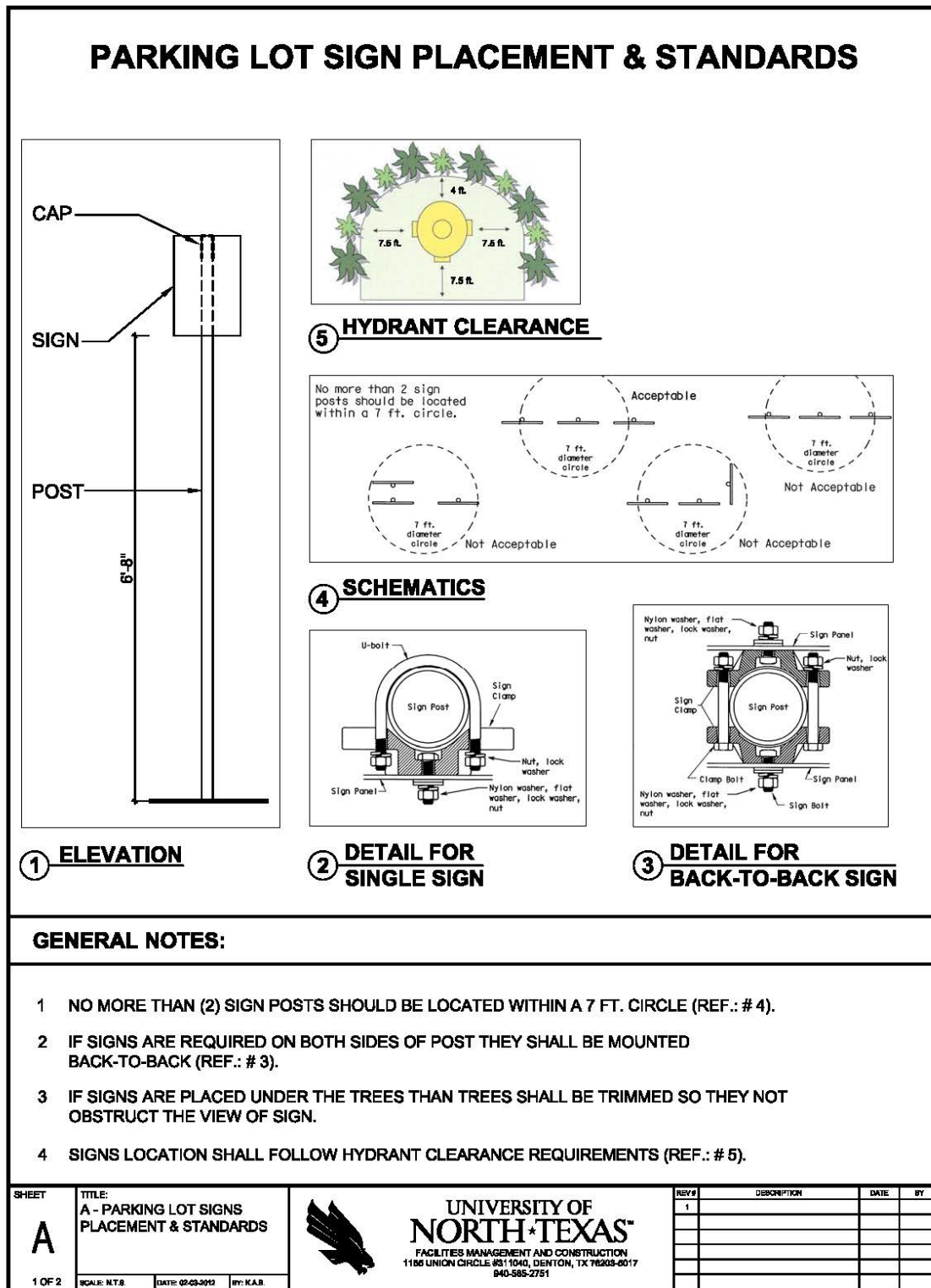
Figure 36 Parking Lot Sign Placement and Standards
