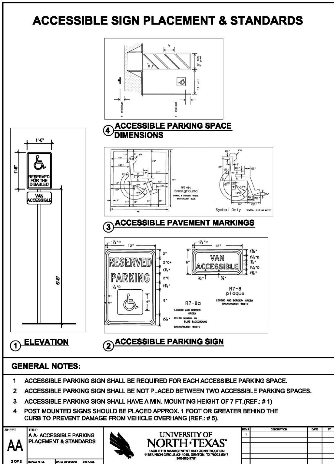
Figure 37 Accessible Sign Placement and Standards
