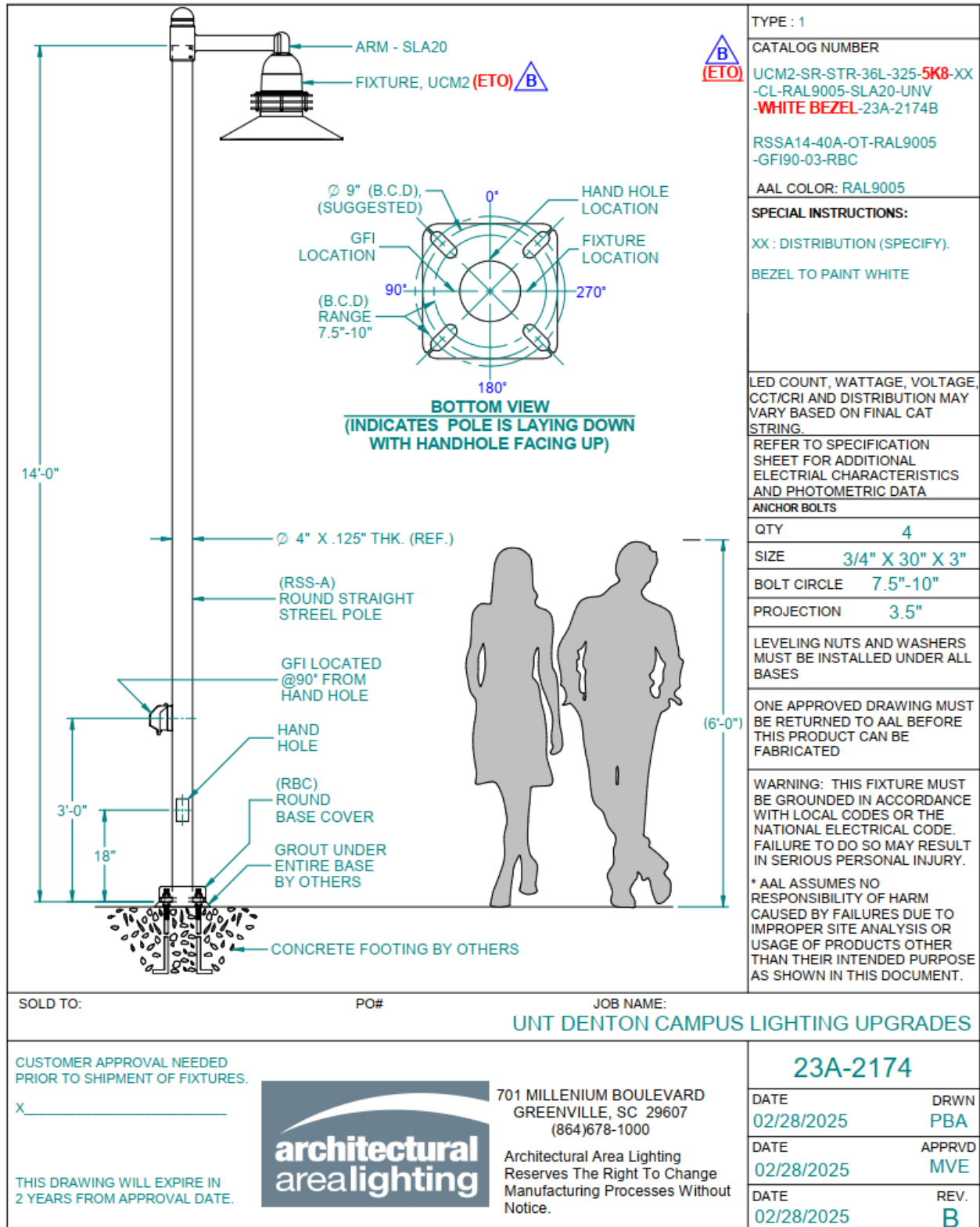
Figure 38 Pedestrian Pole / Fixture
