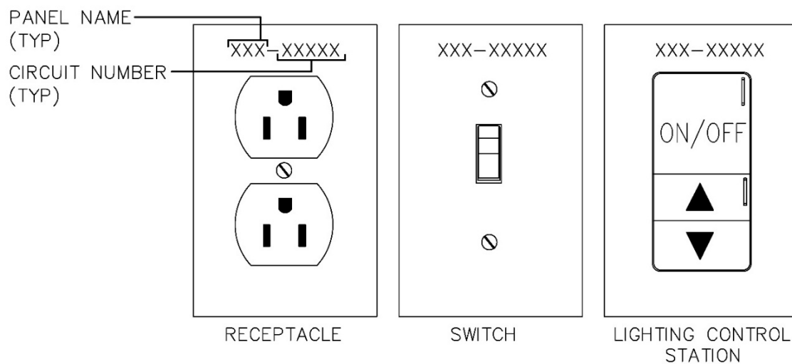
Fig. 26-01 Device Engraving Example
