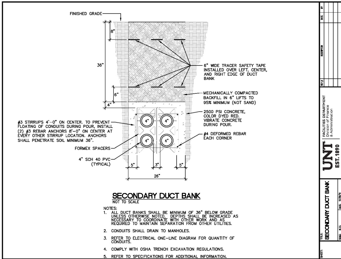
Figure 43 Secondary Power Duct Bank
