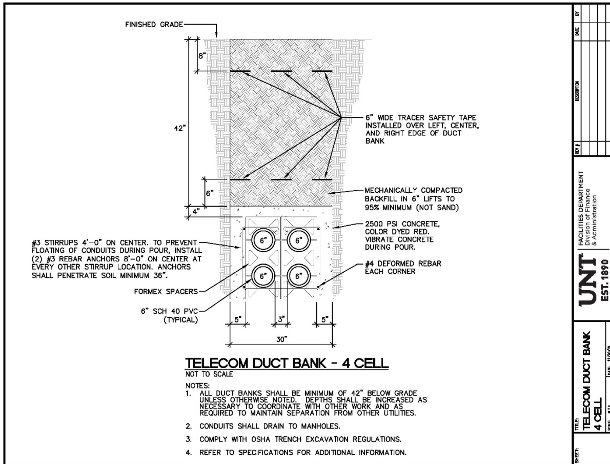
Figure 45 Telecommunications Duct Bank 4 Cell
