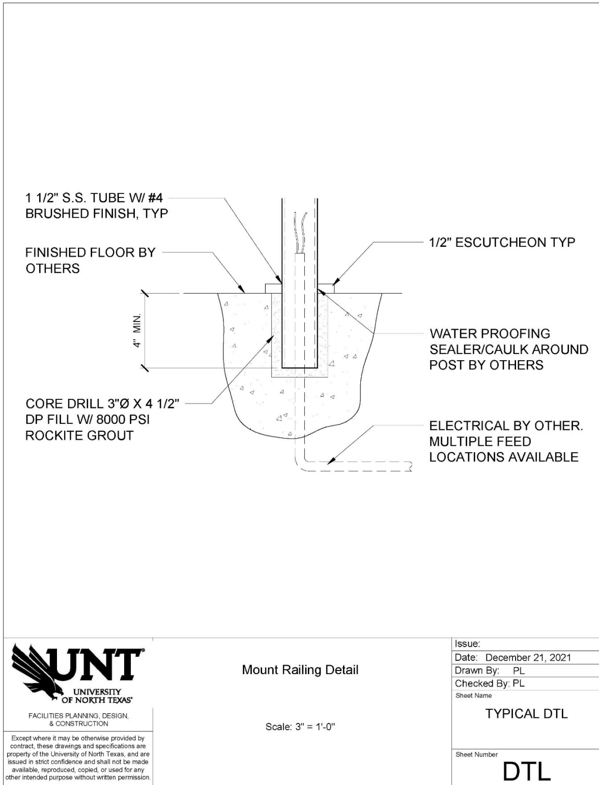
Figure 33 Handrail Detail
