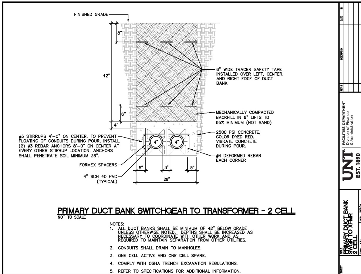
Figure 42 Primary Power Duct bank 2-Cell to Transformer
