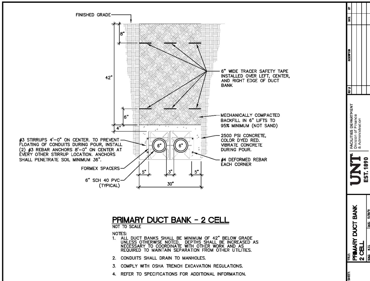
Figure 41 Primary Power Duct Bank 2-Cell
