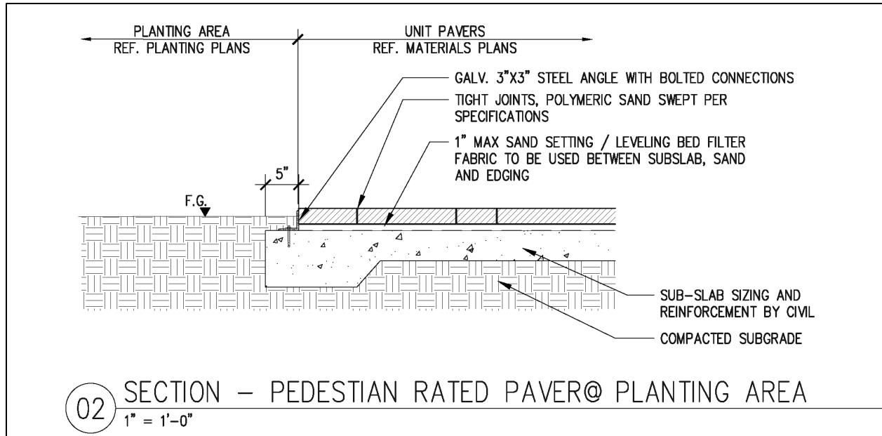
Figure 51 Paver Design
