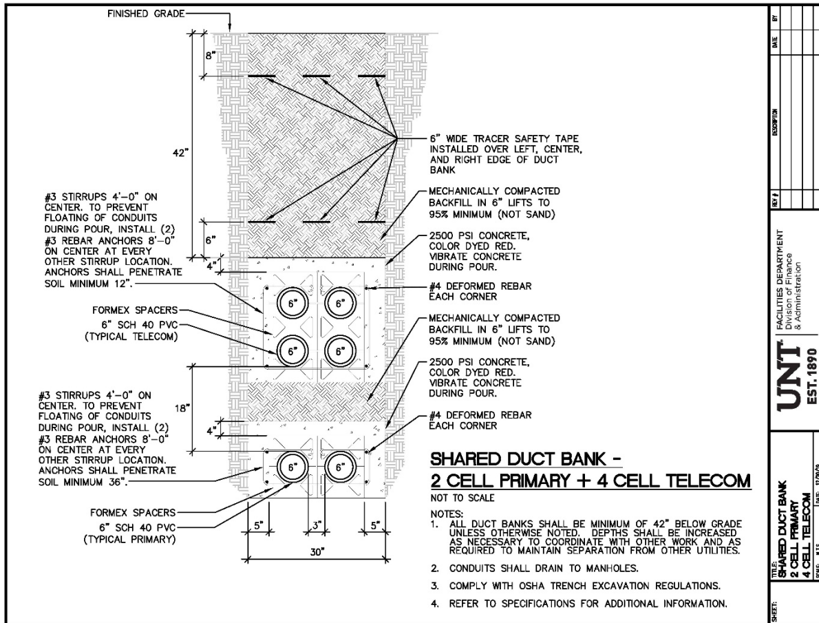
Figure 46A Shared Duct bank 2 Cell Primary &amp; 4 Cell Telecom
