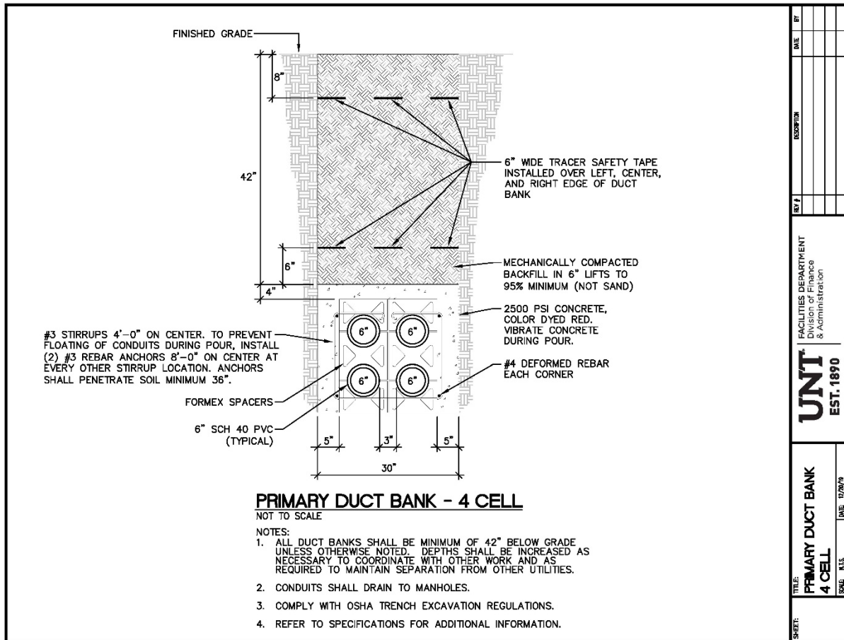
Figure 40 Primary Power Duct bank 4-Cell
