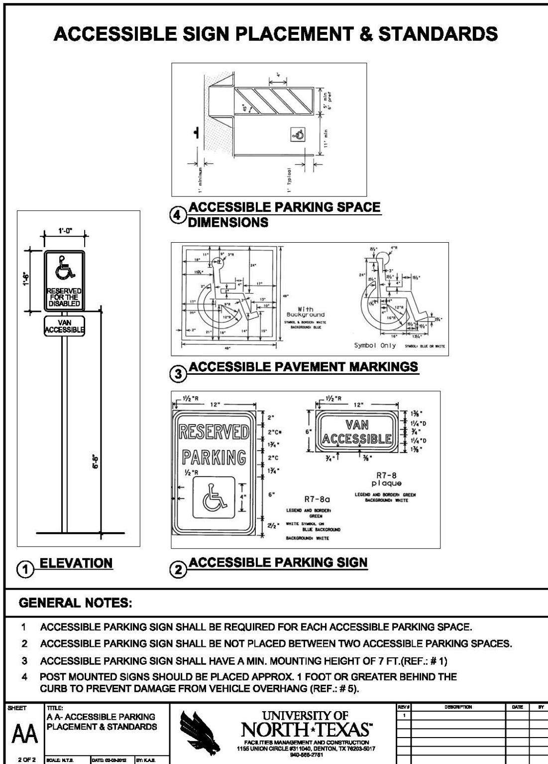
Figure 36 Accessible Sign Placement and Standards
