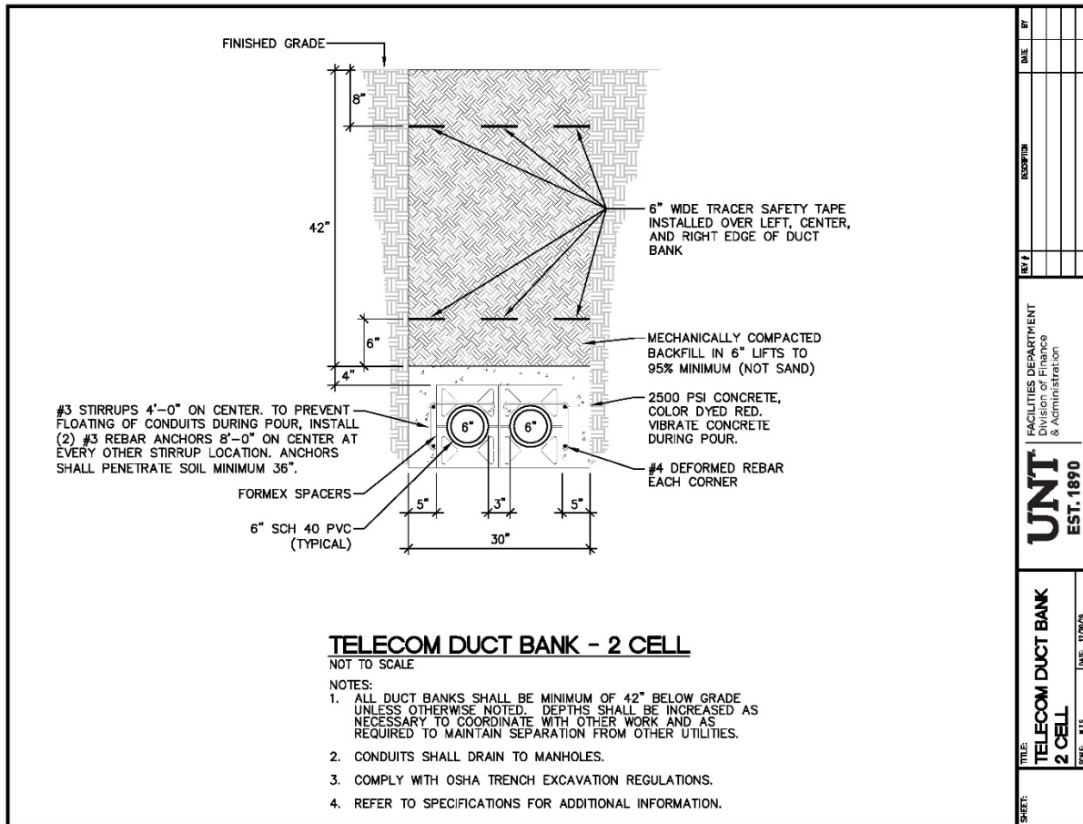
Figure 44 Telecommunications Duct bank
