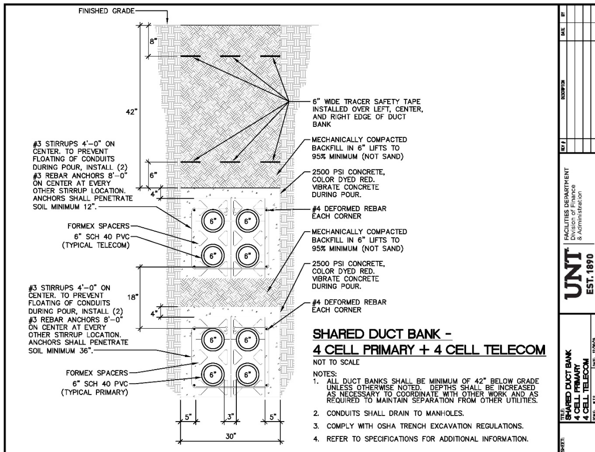
Figure 47B Shared Duct bank 4 Cell Primary & 4 Cell Telecom
