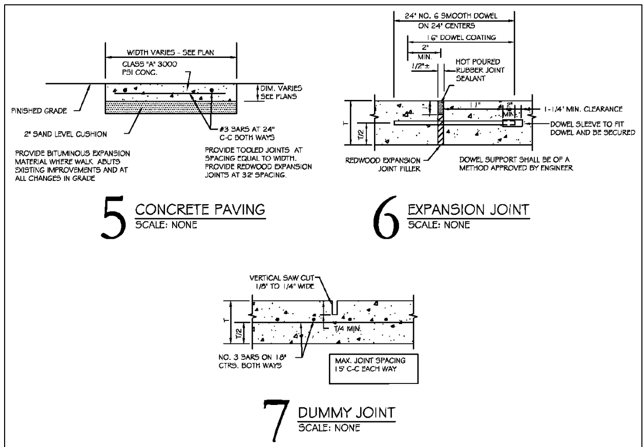
Figure 52 Control and Expansion Joints
