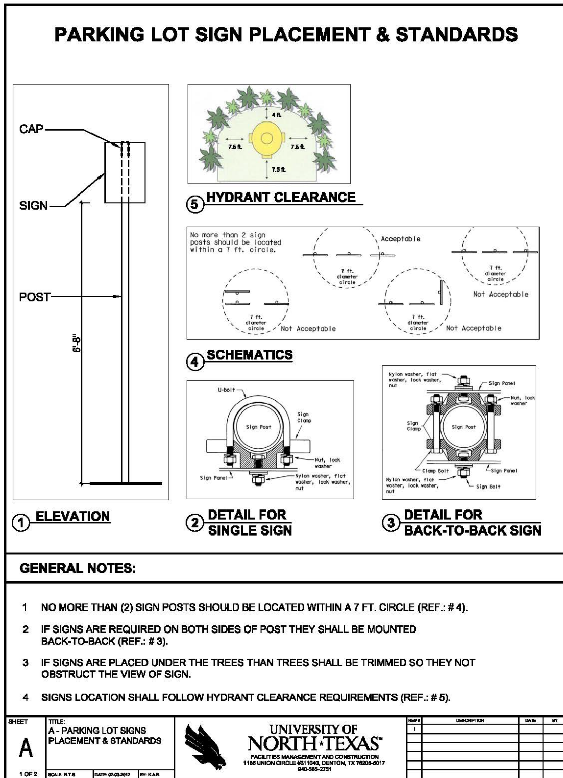
Figure 35 Parking Lot Sign Placement and Standards
