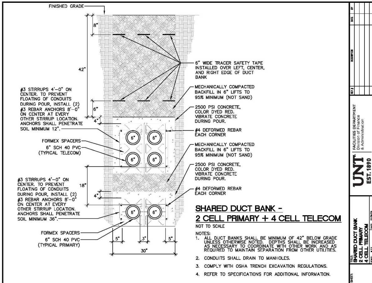
Figure 46A Shared Duct bank 2 Cell Primary & 4 Cell Telecom
