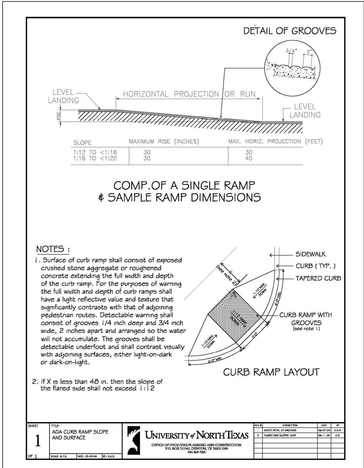
Figure 2 ADA Ramp and Curb Cut Details
